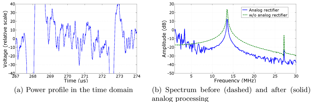
Fig. 5: DES encryption on the Mifare DESFire MF3ICD40
