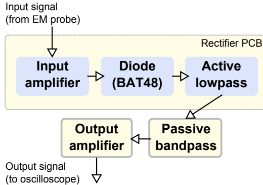
Fig. 2: Structure of the analog demodulation circuitry
