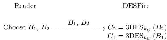
Fig. 3: Excerpt of the Mifare DESFire authentication protocol relevant for SCA
