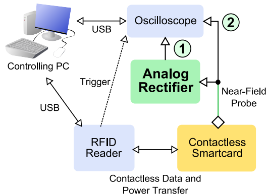
Fig. 1: Overview of measurement environment
