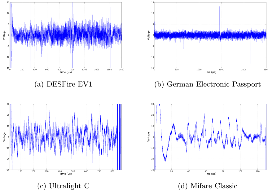
Fig. 9: Power profiles of various contactless smartcards
